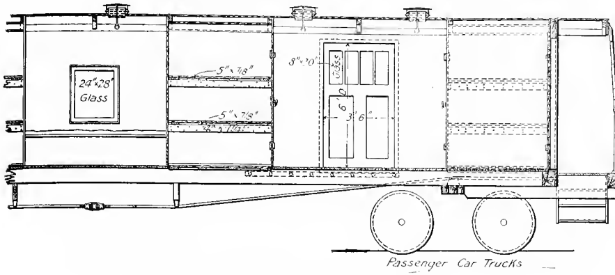
Fig. 271. Part Longitudinal Section.
